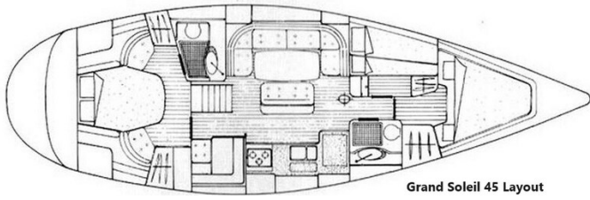
Grand Soleil 45 Layout Cabin
