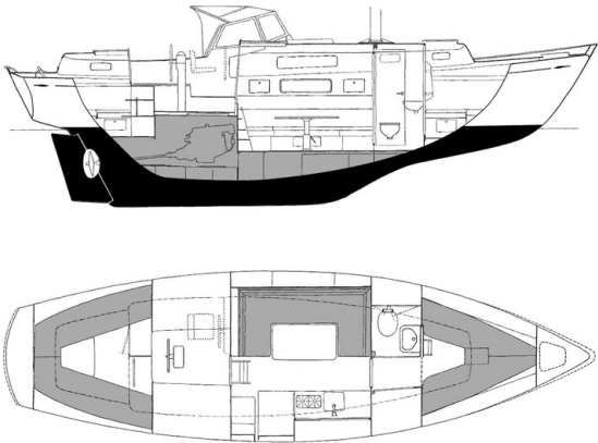
layout HR 35 Rasmus
