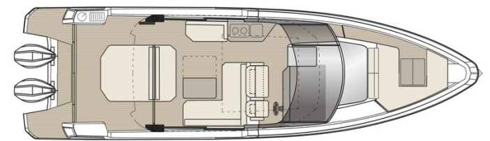
SAXDOR 400 GTC Layout
