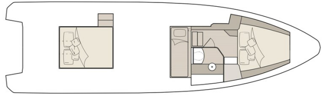
SAXDOR 400 GTC Lower deck
