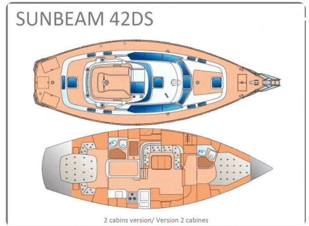
Sunbeam 42 DS-Layout
